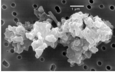
A microscope view of a dust grain
