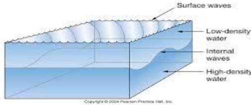
internal and surface waves
